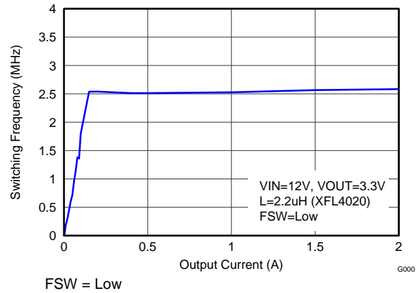
Figure 25. Switching Frequency
