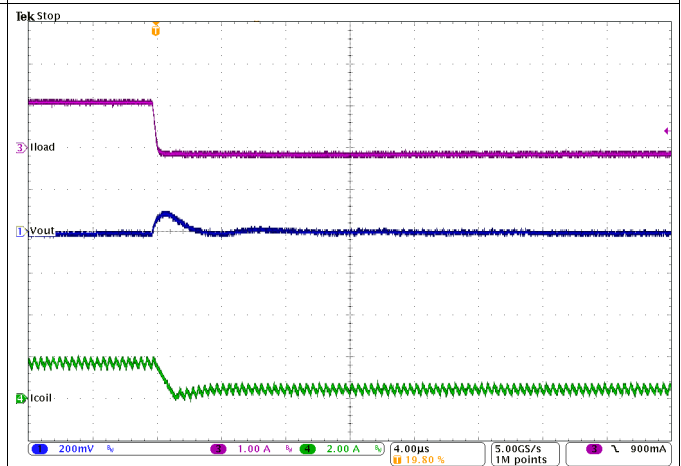
Figure 33. Line Transient Response of Figure 31, Falling Edge
