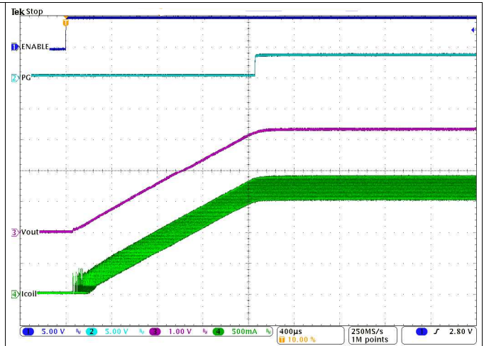
Figure 35. Start-Up into 2 A ( V_{IN} = 12 V , V_{OUT} = 3.3 V )
