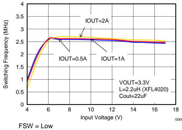
Figure 24. Switching Frequency
