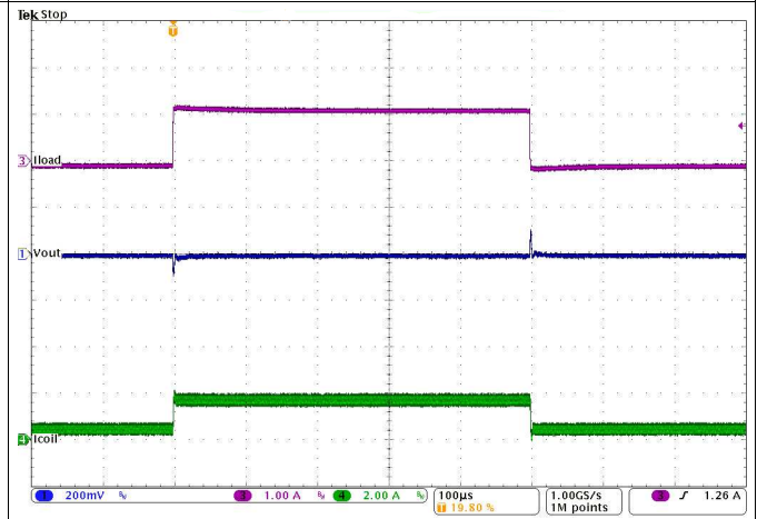
Figure 31. Load Transient Response ( I_{OUT}=0.5 to 2 to 0.5 A, V_{IN} = 12 V, V_{OUT} = 3.3 V)
