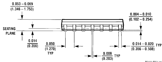
14-Lead Small Outline Molded Package (M) Order Number DM74LS125AM NS Package Number M14A
