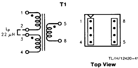
FIGURE 25. Renco RL-5530
