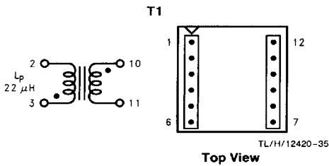
FIGURE 19. Coilcraft Q4435-B (Surface Mount)
