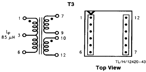
FIGURE 27. Renco RL-5534
