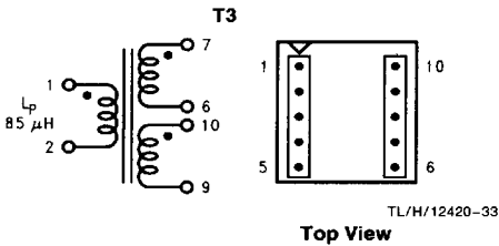
FIGURE 17. Coilcraft Q4343-B
