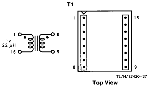
FIGURE 21. Pulse PE-68411 (Surface Mount)
