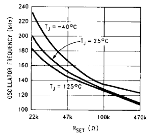
Oscillator Frequency vs Resistance
