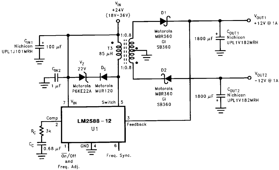
FIGURE 11. Dual-Output Flyback Regulator
