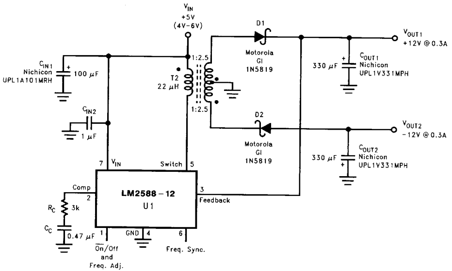
FIGURE 10. Dual-Output Flyback Regulator
