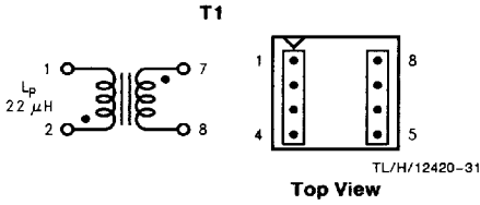
FIGURE 15. Coilcraft Q4434-B
