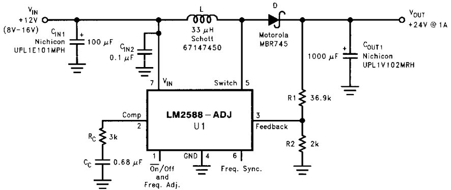
FIGURE 38. +12V to +24V Boost Regulator
