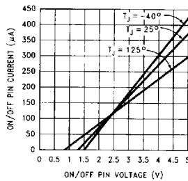
\overline{\text{ON}}/\text{OFF} Pin Current vs Voltage
