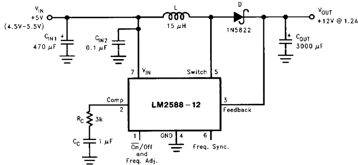
FIGURE 33. 12V Boost Regulator
