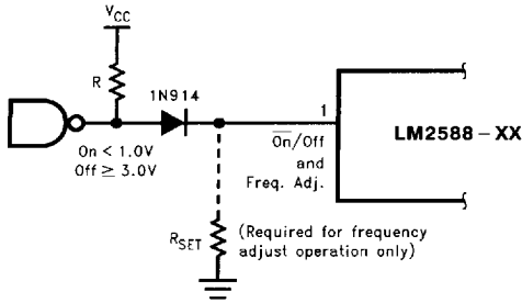
FIGURE 41. Shutdown Operation
