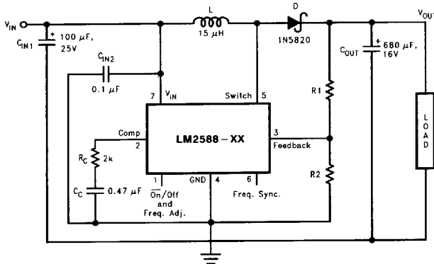
FIGURE 2. LM2588-12 and LM2588-ADJ
