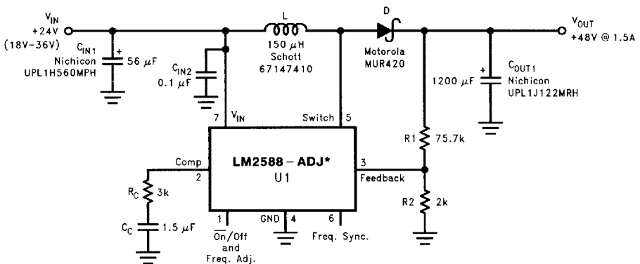
FIGURE 40. +24V to +48V Boost Regulator
