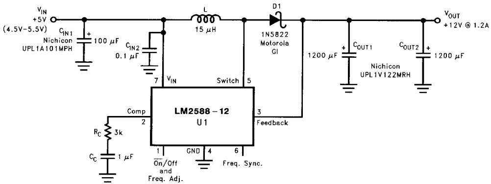
FIGURE 36. +5V to +12V Boost Regulator
