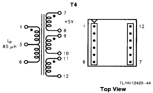
FIGURE 28. Renco RL-5535
