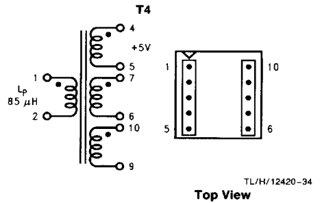
FIGURE 18. Coilcraft Q4344-B
