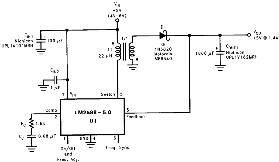
FIGURE 8. Single-Output Flyback Regulator
