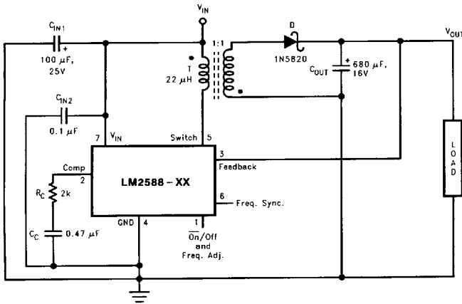
FIGURE 1. LM2588-3.3 and LM2588-5.0
