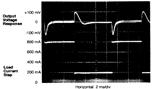
FIGURE 35. V_{OUT} Response to Load Current Step
