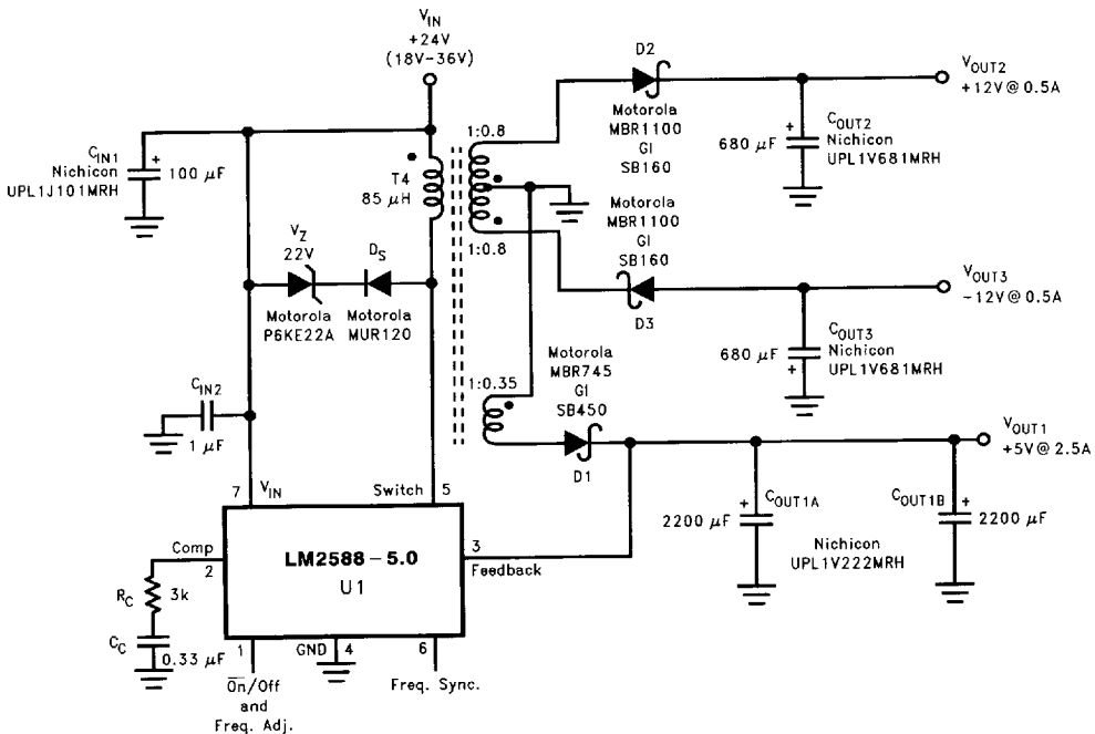
FIGURE 12. Triple-Output Flyback Regulator
