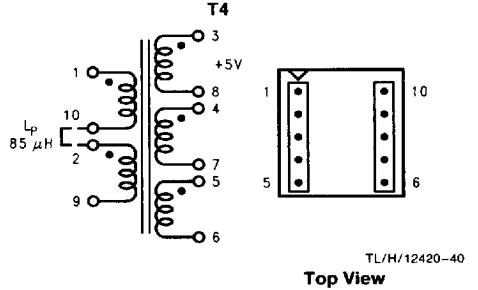
FIGURE 24. Pulse PE-68422 (Surface Mount)
