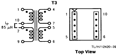
FIGURE 23. Pulse PE-68421 (Surface Mount)
