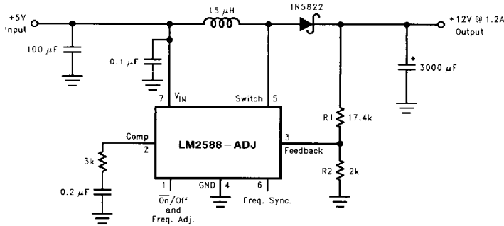
FIGURE 45. Boost Regulator
