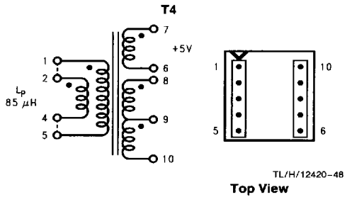
FIGURE 32. Schott 67140930
