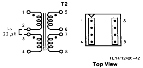
FIGURE 26. Renco RL-5531
