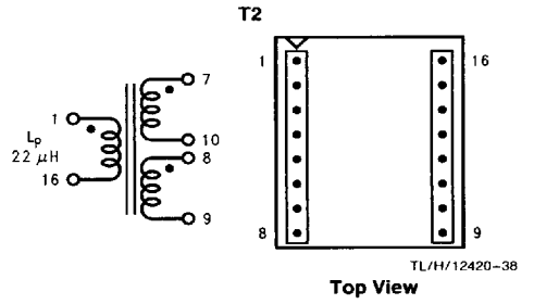
FIGURE 22. Pulse PE-68412 (Surface Mount)
