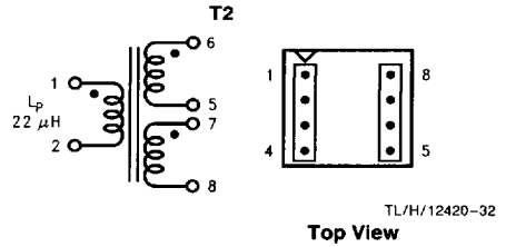
FIGURE 16. Coilcraft Q4337-B
