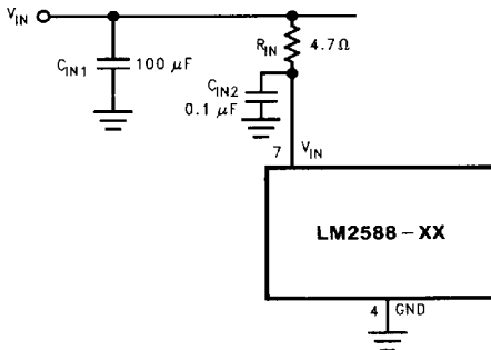
FIGURE 47. Input Line Filter
