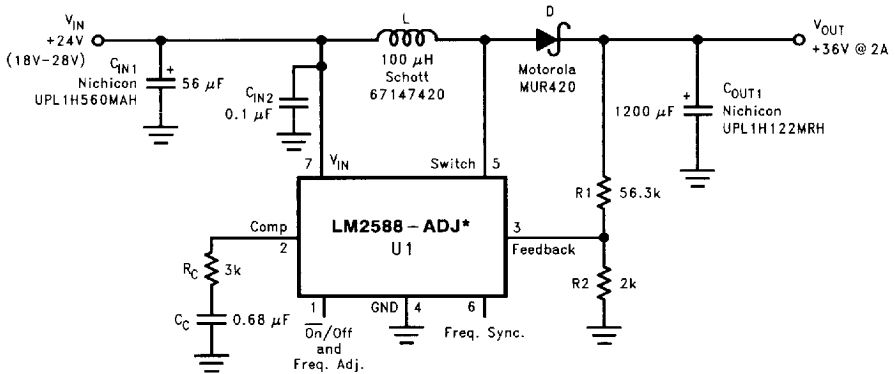
FIGURE 39. +24V to +36V Boost Regulator
