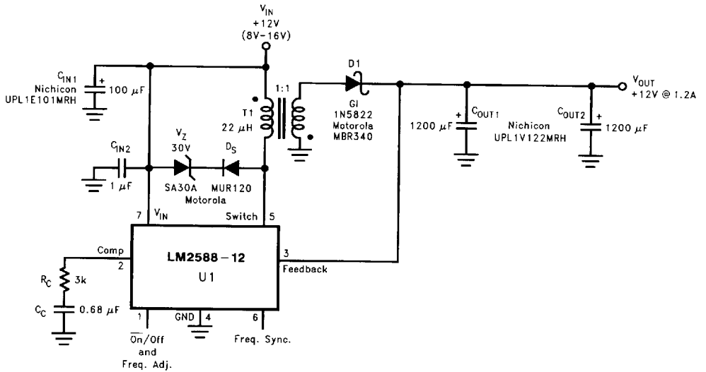
FIGURE 9. Single-Output Flyback Regulator
