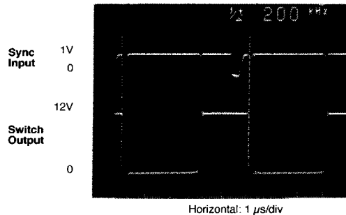
FIGURE 44. Waveforms of a Synchronized 12V Boost Regulator
