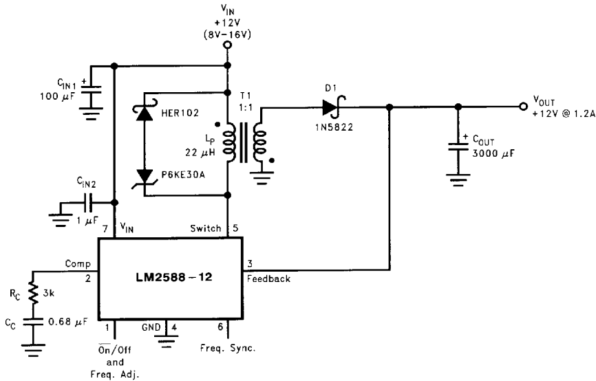
FIGURE 4. 12V Flyback Regulator Design Example
