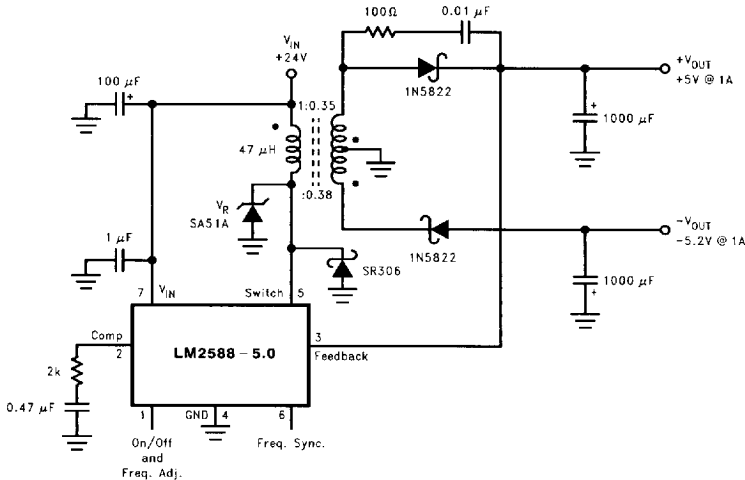
FIGURE 46. Flyback Regulator
