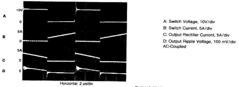
FIGURE 5. Switching Waveforms
