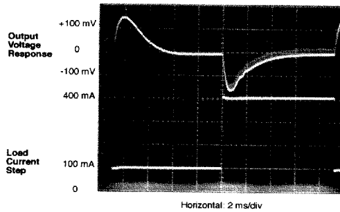
FIGURE 6. V_{OUT} Response to Load Current Step
