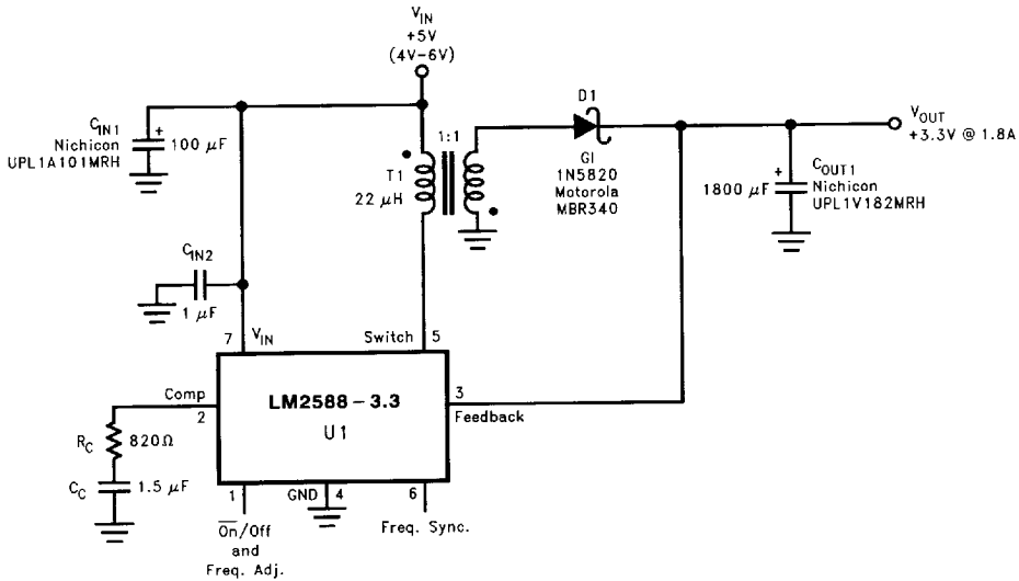
FIGURE 7. Single-Output Flyback Regulator
